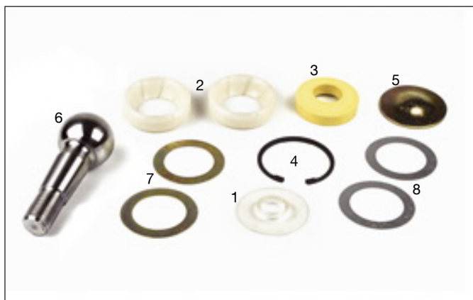
080.536 5001 832 613 - (4090 435 642) Repair Kit Axle Rod With Bolt M30x2xø65x169.5
